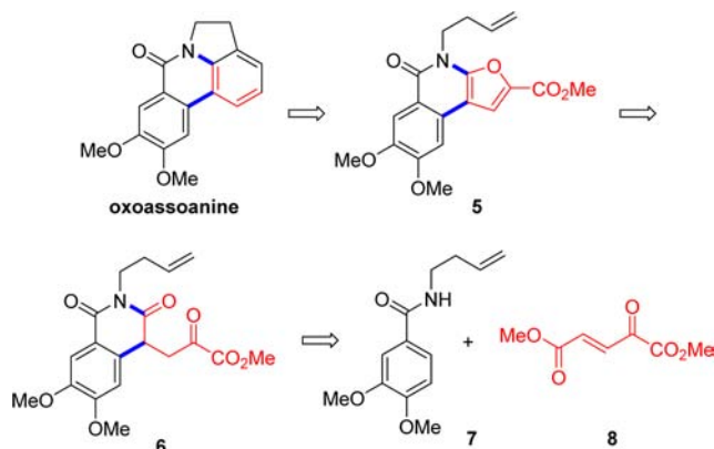
Scheme 5. Synthesis of Oxoassoanine
