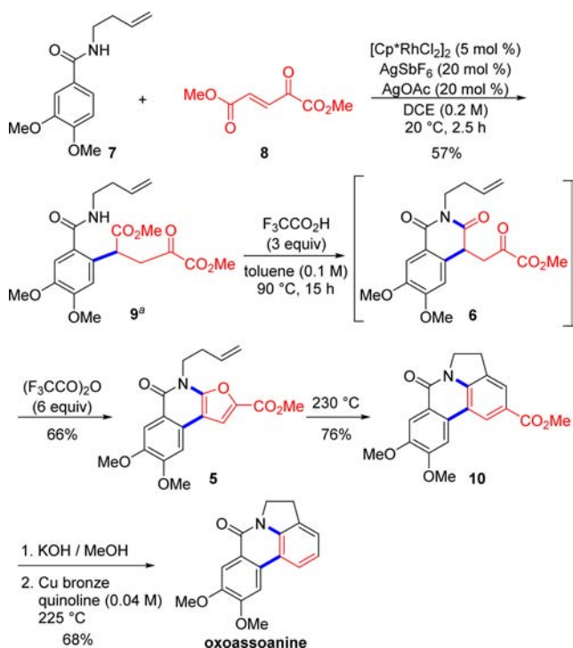
Scheme 5. Synthesis of Oxoassoanine
