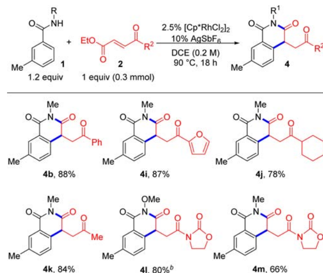
Scheme 3. Evaluation of Electrophilic Olefin Substrate Scope a
