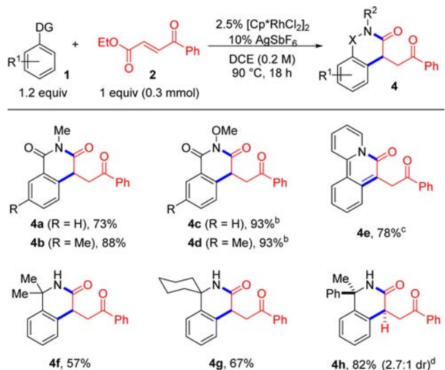
Scheme 2. Evaluation of Directing Group Substrate Scope a
